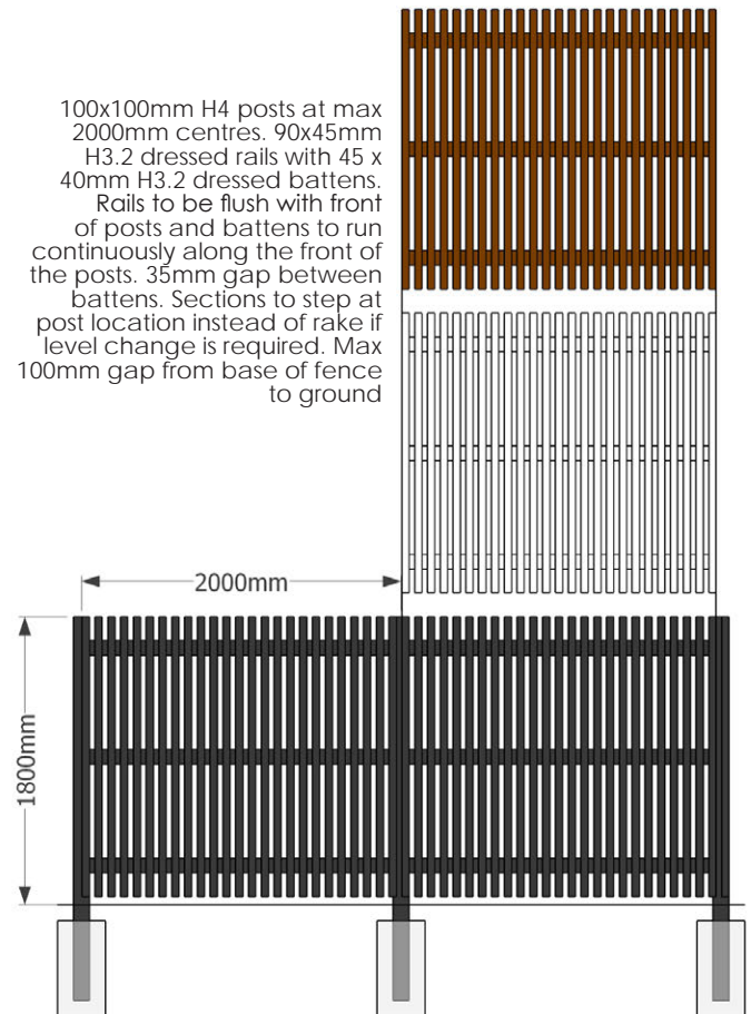
1.8m SCREEN FENCE TYPE A + B
